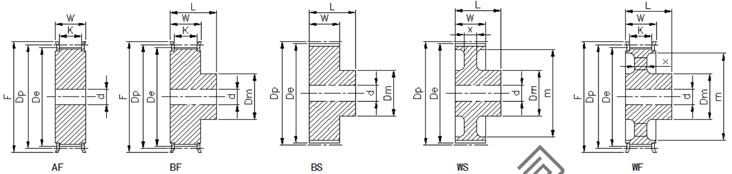
8M型标准皮带宽85mm
